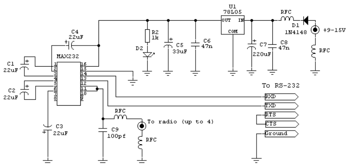
Icom CT-17 Interface
